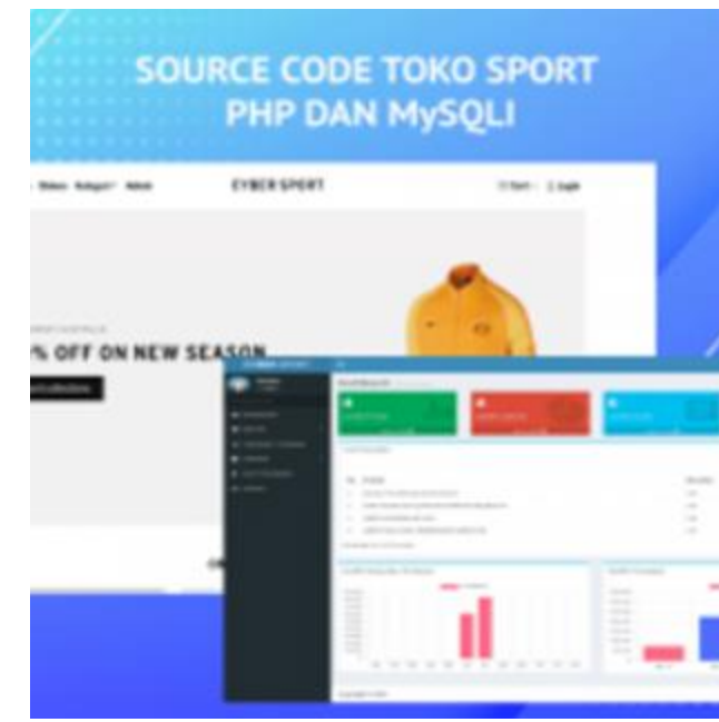
SOURCE CODE
